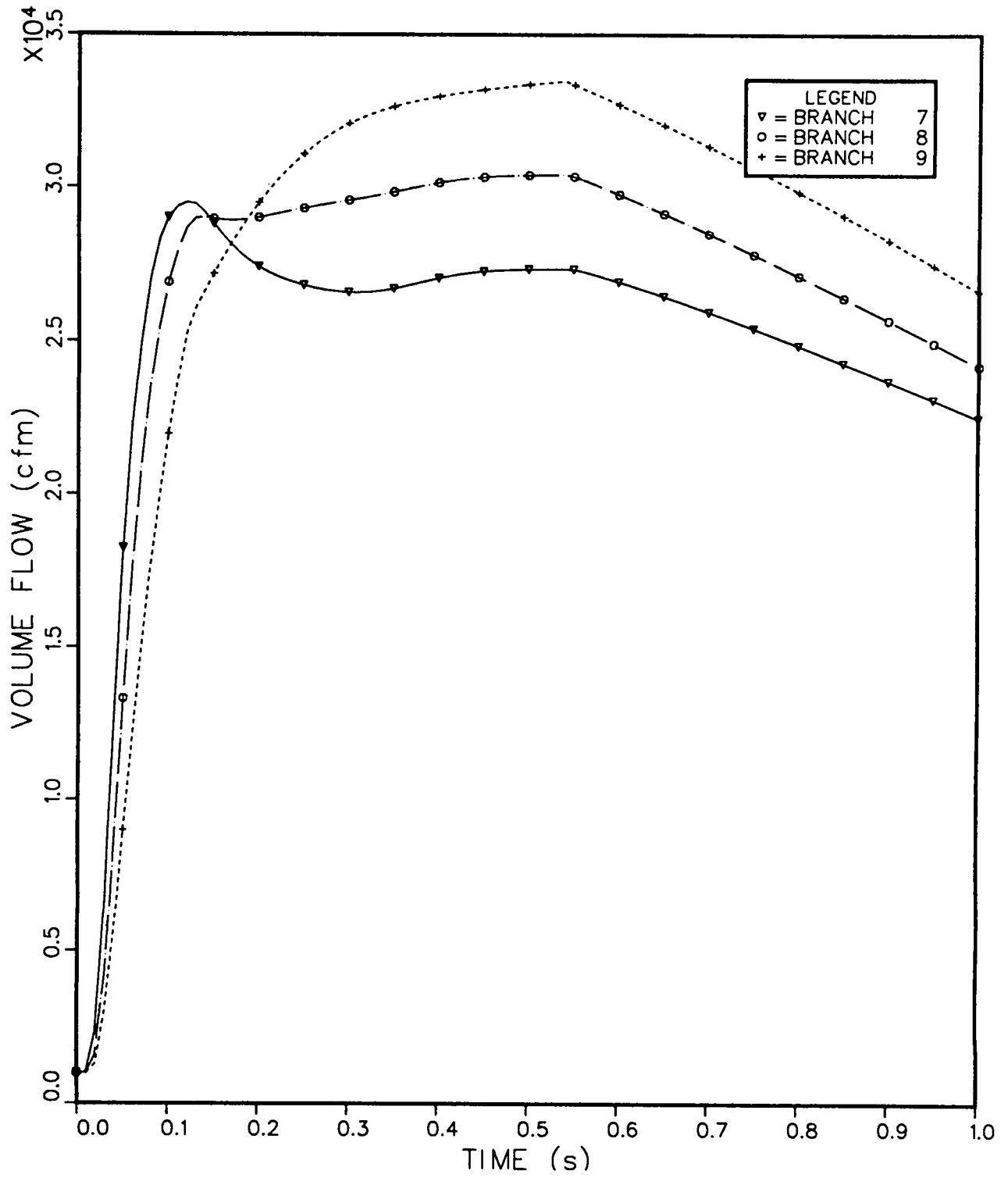
Fig. 21. Volume flows.
