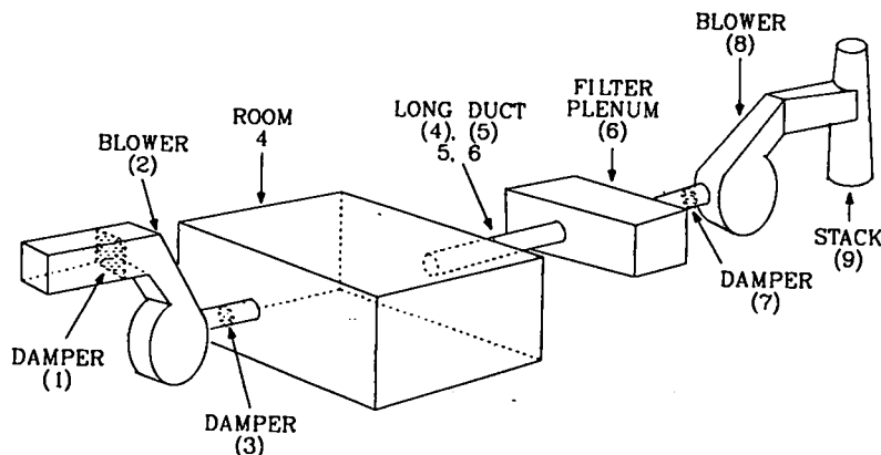
Fig. 12. Ventilation system for sample problem.
